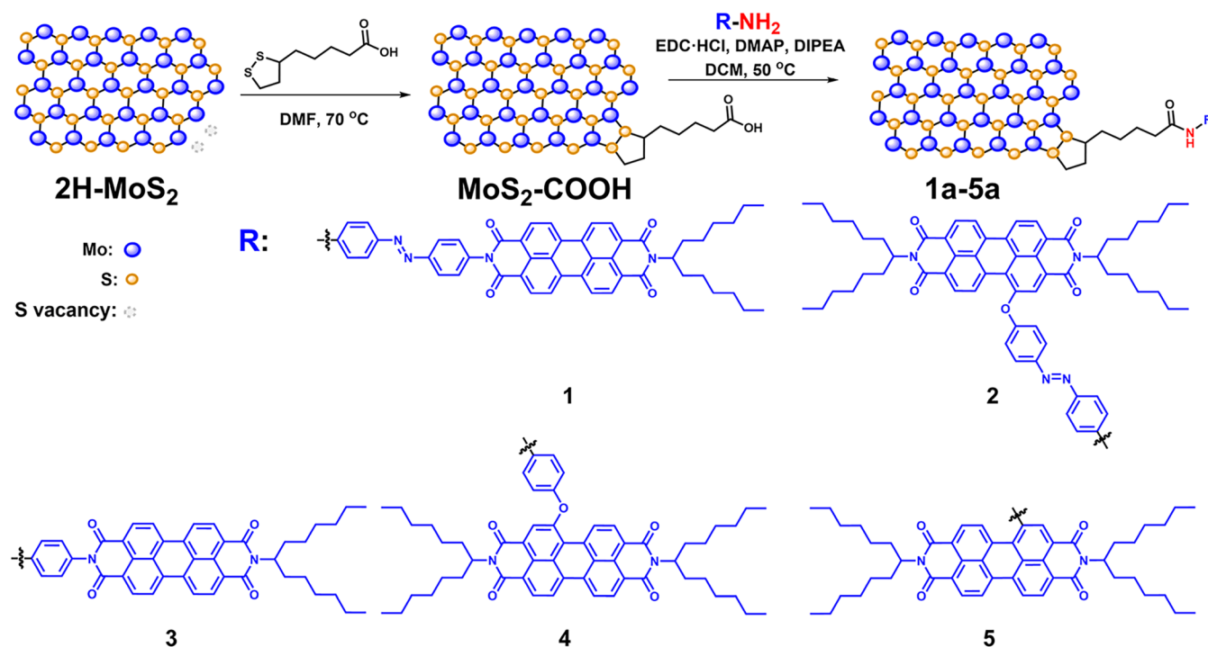
Figure 1. Illustrative preparation of MoS 2 -PDI hybrid materials 1a–5a.
