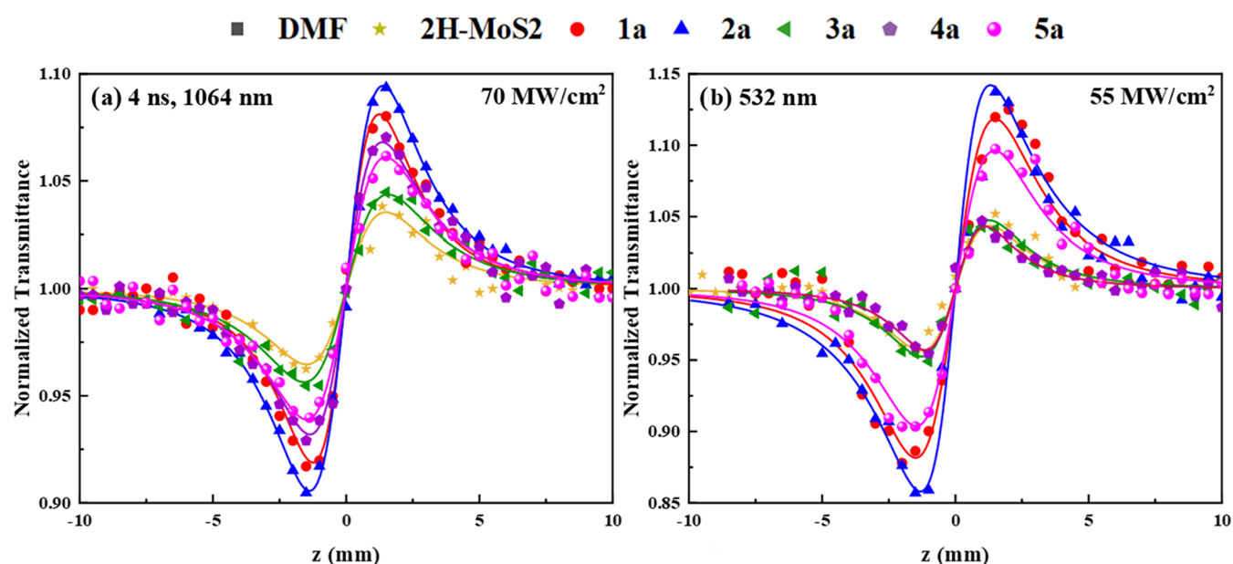
Figure 7. “Divided” Z-scans of MoS 2 –PDI hybrid materials 1a – 5a in DMF (0.1 mg/mL) under 4 ns (a) 1064 and (b) 532 nm laser excitation.
