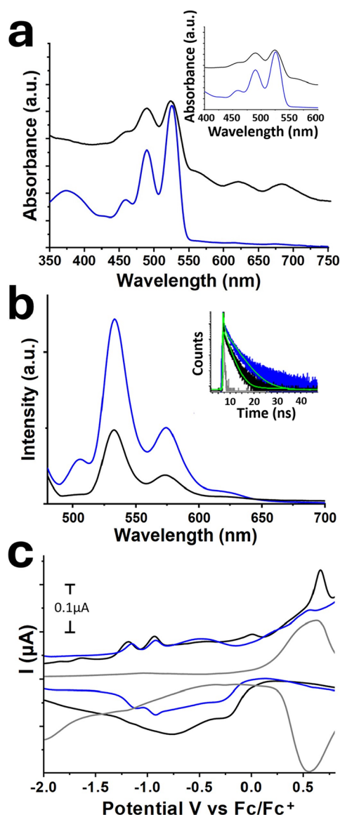
Figure 4. (a) UV-vis spectra of PDI derivative 1 (blue) and MoS 2 -PDI hybrid material 1a (black), obtained in dichloromethane. Inset: UV-vis spectrum of MoS 2 -PDI hybrid material 1a, after subtraction of absorbance due to MoS 2 (black), in comparison with the same optical concentration spectrum of PDI derivative 1 (blue). (b) Emission spectra (excitation at 440 nm) of PDI derivative 1 (blue) and MoS 2 -PDI hybrid material 1a (black), obtained under equal optical absorbance at the excitation wavelength in dichloromethane. Inset: Emission decay of PDI derivative 1 (blue), MoS 2 -PDI hybrid material 1a (black), and the corresponding fitting (green). (c) Square-wave pulse voltammetry graphs of exfoliated MoS 2 (gray), PDI derivative 1 (blue), and MoS 2 -PDI hybrid material 1a (black) in dry DMF, with 0.1 M tetrabutylammonium hexafluorophosphate as the electrolyte.
