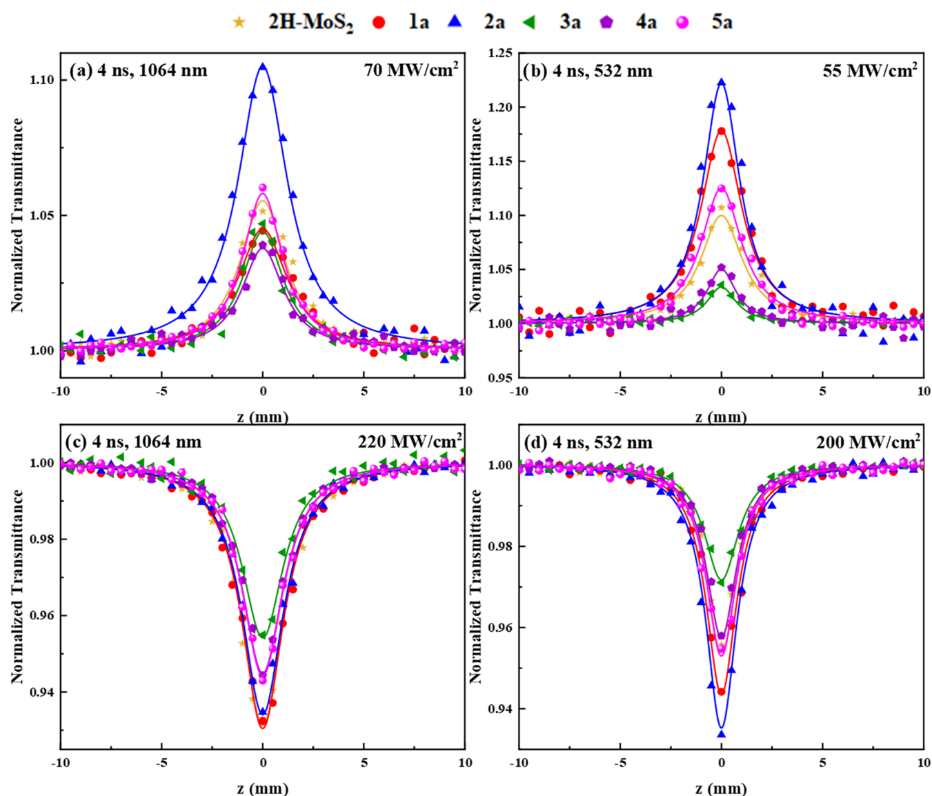
Figure 6. OA Z-scans of MoS 2 –PDI hybrid materials 1a–5a in DMF (0.1 mg/mL), under 4 ns, 1064 and 532 nm laser excitation, using low (a, b) and high (c, d) laser intensities.
