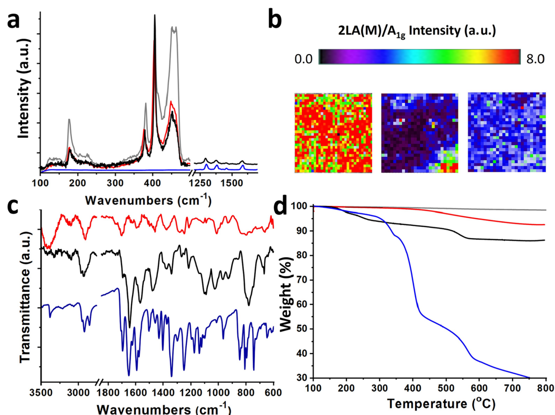
Figure 2. (a) Raman spectra (633 nm) of PDI derivative 1 (blue), exfoliated MoS 2 (gray), MoS 2 -COOH (red), and MoS 2 -PDI hybrid material 1a (black). (b) Raman spectral maps of the 2LA(M)/A 1g ratio for exfoliated MoS 2 (left), MoS 2 -COOH (center), and MoS 2 -PDI hybrid material 1a (right). (c) IR spectra and (d) TGA graphs of PDI derivative 1 (blue), MoS 2 -COOH (red), and MoS 2 -PDI hybrid material 1a (black).
