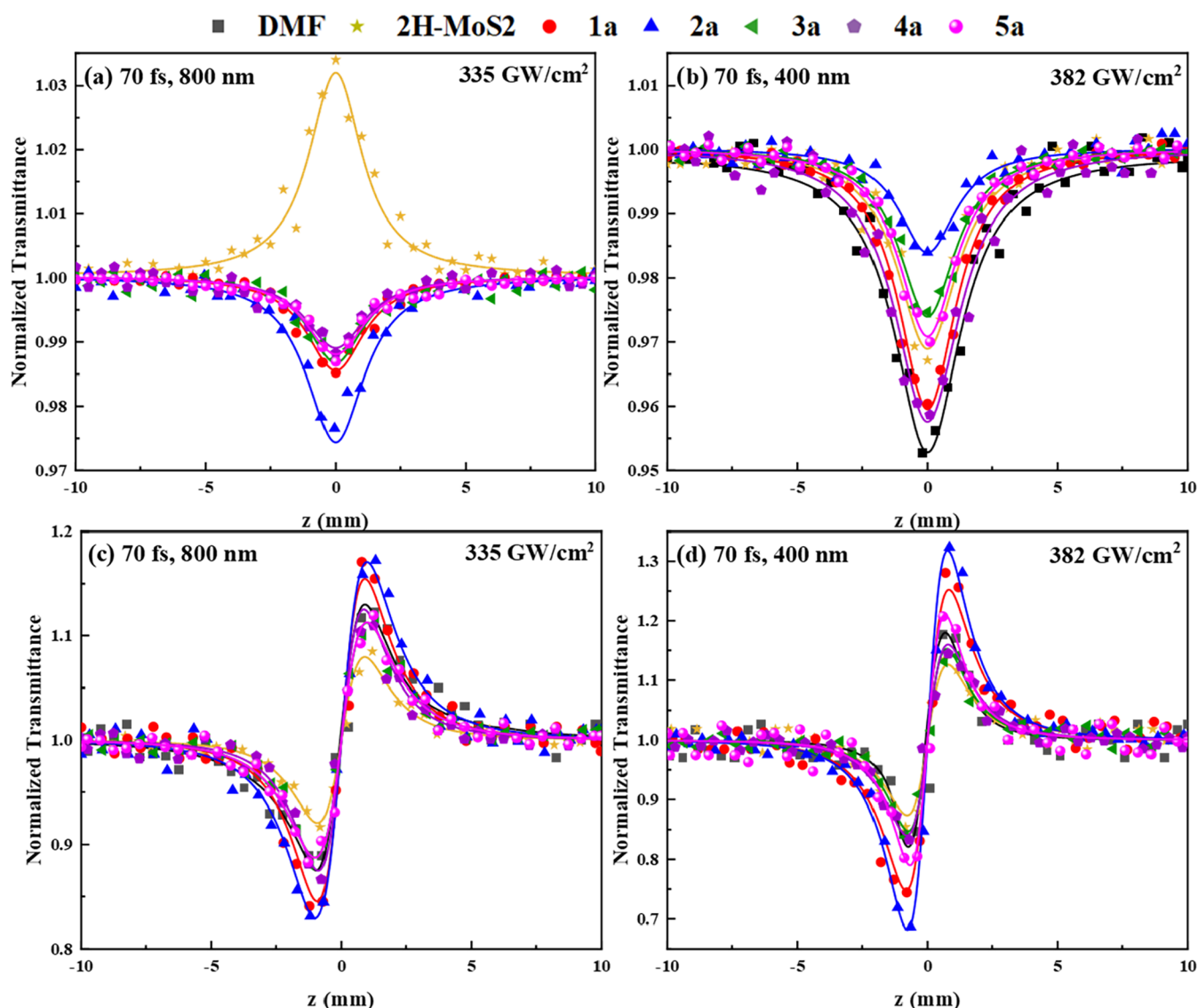
Figure 10. (a, b) OA and (c, d) “divided” Z-scans of MoS 2 –PDI hybrid materials 1a–5a in DMF (0.1 mg/mL), under 70 fs, 800 and 400 nm laser excitation.
