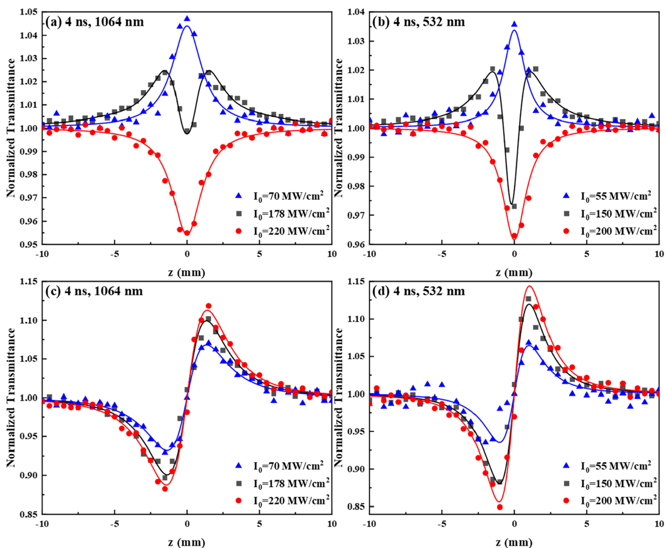
Figure 5. (a, b) OA and (c, d) “divided” Z-scans of MoS 2 –PDI hybrid material 3a in DMF (0.1 mg/mL) obtained under 1064 and 532 nm excitation, using different laser intensities.
