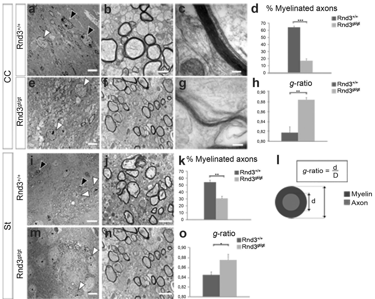
Fig. 3 The absence of Rnd3 expression alters the organization of the myelin sheath in the CC and St. Representative electron micrographs of the CC in wt ( a–c ) and Rnd3 gt/gt mice ( e–g ) at different magnifications. In wt animals, mature OLC (black arrowheads) were abundant ( a ), but in RhoE gt/gt brains the presence of more immature precursors (white arrowheads) was consistently detected ( e ). Myelinated axons show a higher myelin compaction in wt than in Rnd3 gt/gt mice. c, g The details of the myelin compaction in wt and Rnd3 gt/gt mice, respectively. Representative electron micrographs of the St in wt ( i–j ) and Rnd3 gt/gt mice ( m–n ) at different magnifications. Black arrowheads indicate mature OLC and white arrowheads indicate immature OLC. The total number of myelinated axons and the myelin thickness are reduced in the CC and the St of Rnd3 gt/gt mice. The percentage
