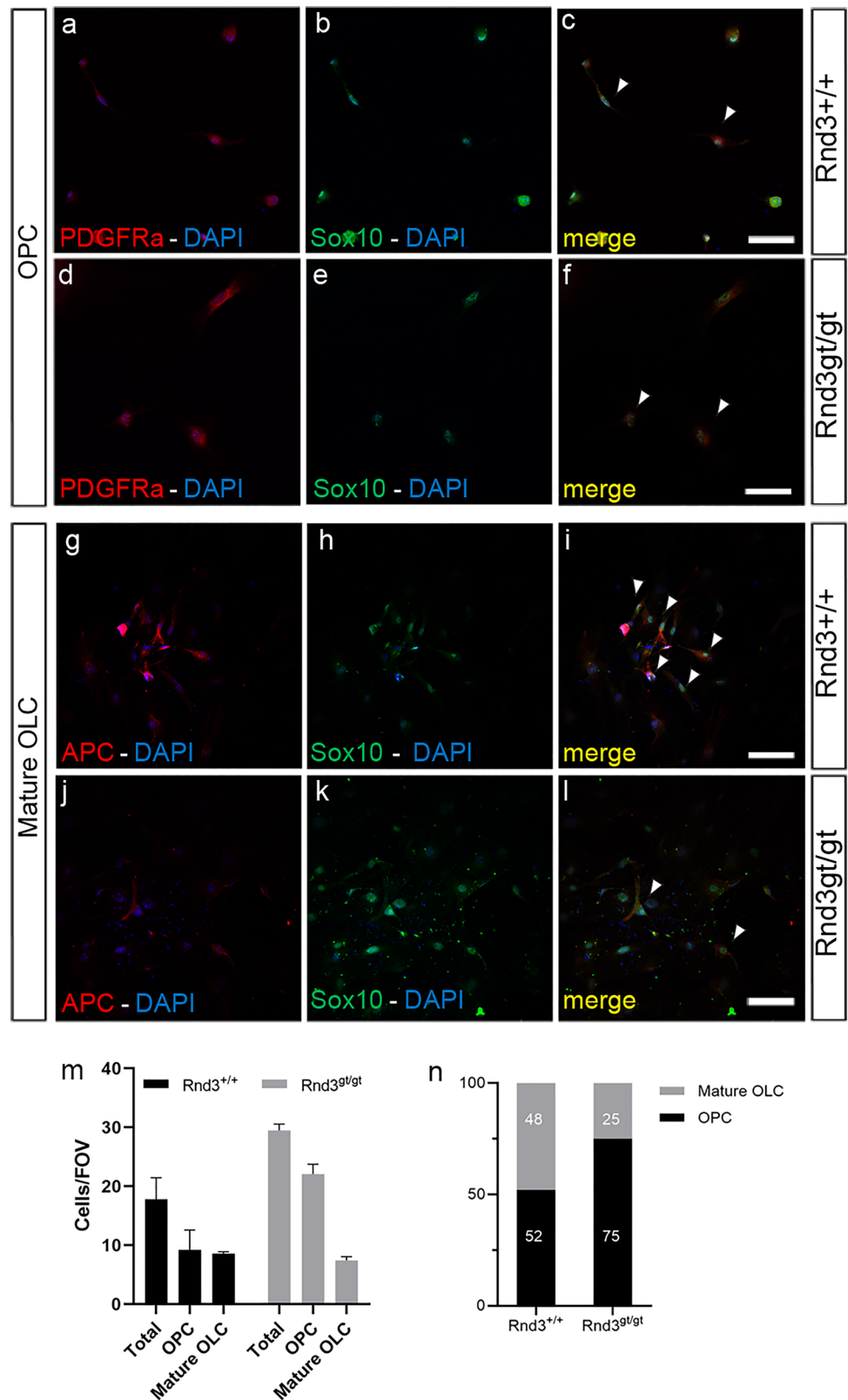
Fig. 6 Rnd3 deficiency alters the differentiation of oligodendrocytes in vitro. Undifferentiated cultures showed that most Sox10-IR cells (green) were positive for PDGFR \alpha (red), both in control and Rnd3 gt/gt cultures (a–c and d–f, respectively). Differentiated OLCs are Sox10+/APC+/+ (g–i). Scale Bar a–f: 50 \mu m; g–i: 100 \mu m. In (m), the number of Sox10+ (Total) Sox10+/APC– (OPCs), Sox10+/APC+ (OLCs) cells per field of view (FOV) at the end of the differentiation protocol is shown. Columns represent the mean value + SEM of cultures obtained from three different animals of each genotype. At least nine different 20X FOV were counted from each culture. In (n), the percentage of OPCs (Sox10+/APC–) and mature OLCs (Sox10+/APC+) when compared to the total number of Sox10+ cells is shown
