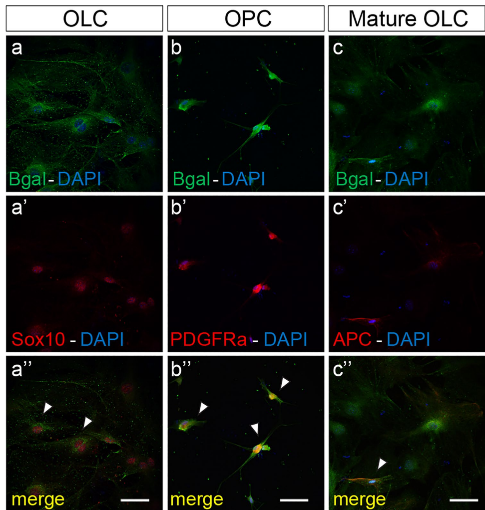
Fig. 5 Rnd3 is expressed during the differentiation process of OLCs in vitro. ICC of different OLC markers in the differentiation culture medium conditions showed Rnd3 expression ( \beta gal+, green) in all differentiation stages: in a–a'' , total OLC lineage (Sox10 positive); in b–b'' , OPCs (PDGFRa positive); in c–c'' , mature OLCs (APC positive). In all images, blue staining corresponds to the nuclei (DAPI). OPC oligodendrocyte precursor cells, OLC oligodendrocytes. Scale bar: 50 \mu m
