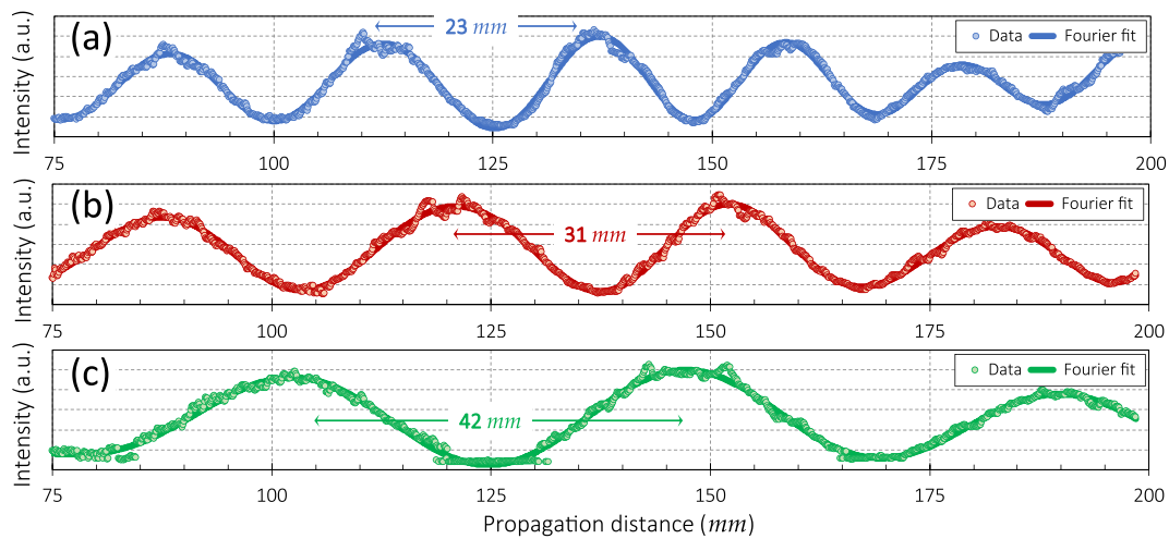
Fig. 4. Intensity along the propagation distance with the LC axicon tuned with (a) (2.5, 0.5) V_{rms} , (b) (3.0, 0.5) V_{rms} and (c) (3.5, 0.5) V_{rms} . The arrows indicate the expected periods for the three cases.
