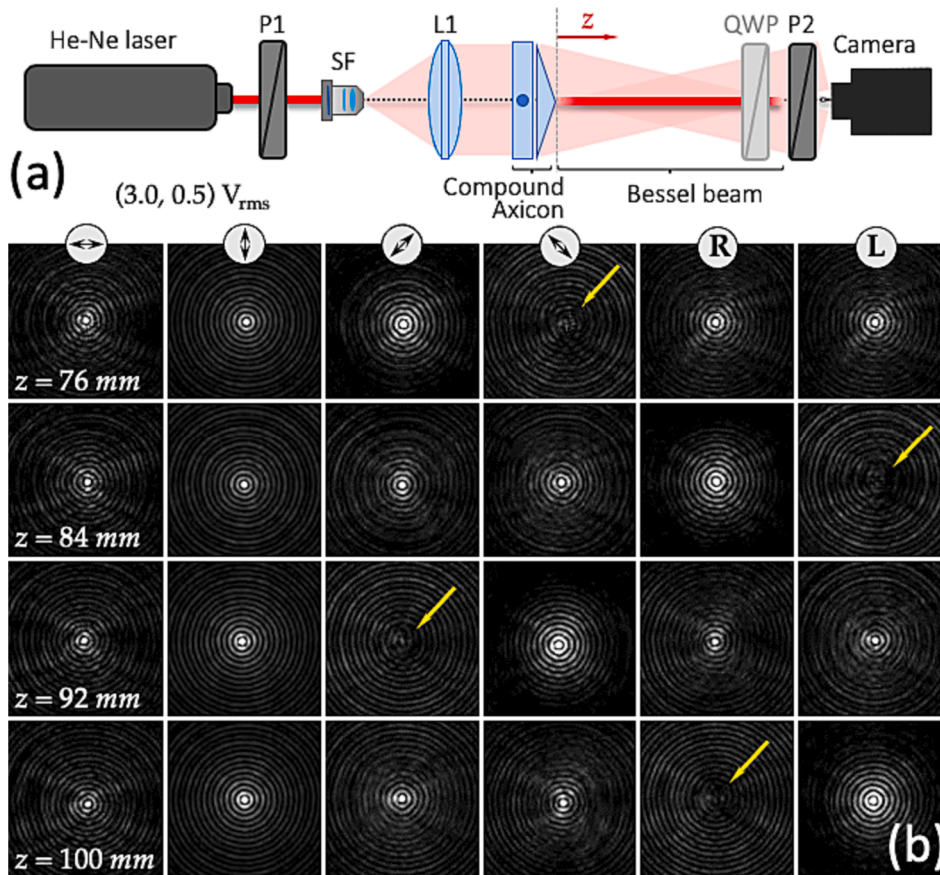
Fig. 3. (a) Optical system for analyzing the Bessel beam generated with the compound axicon, where z denotes the axial distance from the compound axicon. (b) Experimental captures at four axial distances for six different polarization analyzers and applied voltages (3.0, 0.5) V_{rms} . Yellow arrows indicate the situations where the center of the Bessel beam is extinguished. (For interpretation of the references to colour in this figure legend, the reader is referred to the web version of this article.)
