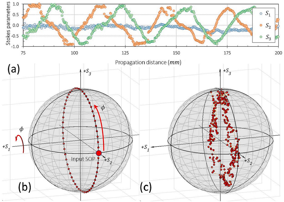
Fig. 5. (a) Experimentally measured normalized Stokes parameters as a function of the propagation distance for case (3.0, 0.5) V_{\text{rms}} . (b) Ideal theoretical SOP trajectory in the Poincaré sphere along propagation. (c) Experimental SOP trajectory derived from the data in (a).
