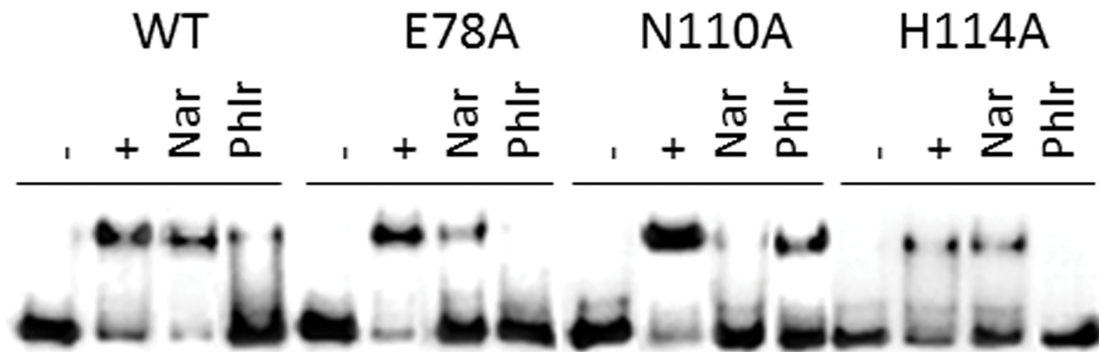
Fig 5. Effect of naringenin and phloretin on the dissociation of TtgR WT and variants (TtgR H114A , TtgR N110A and TtgR E78A ) from ttgR-ttgABC intergenic region by EMSA. (-) 1nM of free labeled operator DNA, (+) DNA-complex with 2 \mu M of TtgR WT and its variants, and DNA complex in the presence of 5 \mu M of naringenin (Nar) and phloretin (Phlr).
