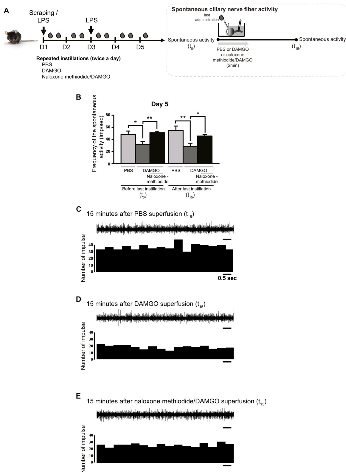
Fig. 5. Repeated topical instillations of DAMGO prevents the increase in spontaneous activity of ciliary nerve fibers induced by corneal pain.
