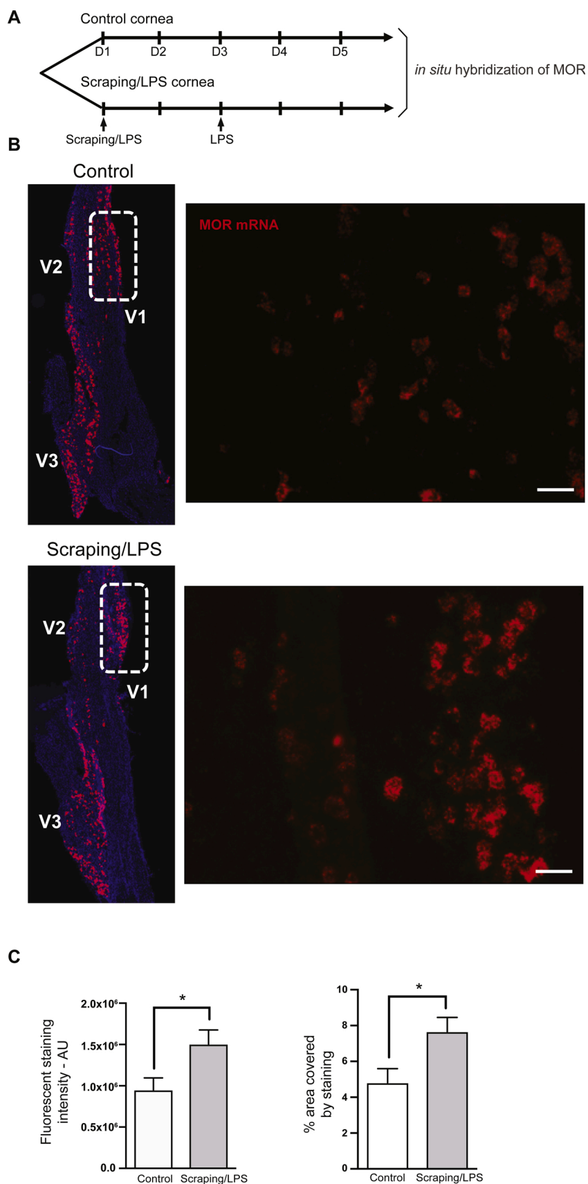
Fig. 4. Mu opioid receptor RNA expression increases in the trigeminal ganglion during inflammatory corneal pain.
