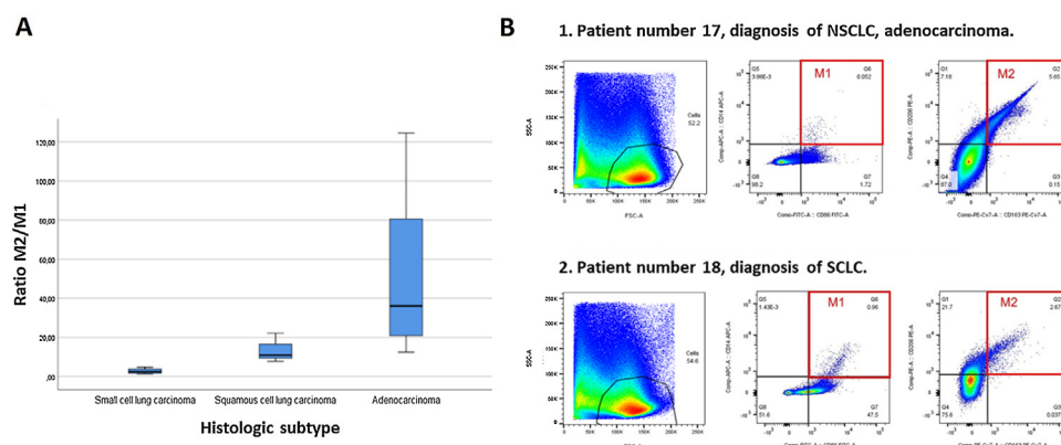
Fig. 1. Characterization of alveolar macrophage populations. (A) M2/M1 ratio according to definitive diagnosis. (B) Different examples of flow cytometry of included patients. SCLC: small cell lung cancer, SSC: side scatter channel, FSC: forward scatter channel.
