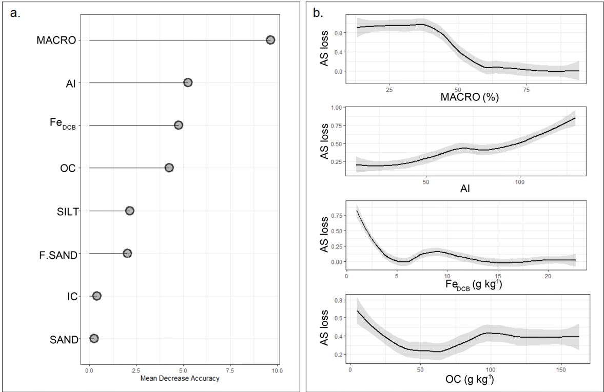
Fig. 7. A. accuracy plot of the main variables regulating as loss; b. partial dependance plots of selected variables.
