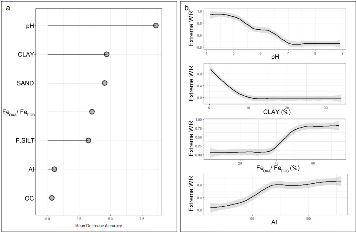
Fig. 6. A. accuracy plot of the main variables regulating extreme wr expression; b. partial dependance plots of selected variables.
