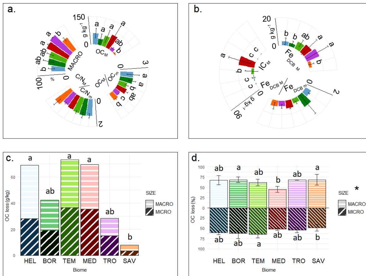
Fig. 3. Main properties of the soil size fractions. a. Polar plot with MACRO content (%), \text{OC}_M content ( \text{g kg}^{-1} ), \text{OC}_M/\text{OC}_m , \text{C/N}_M/\text{C/N}_m ; b. polar plot with \text{IC}_M content ( \text{g kg}^{-1} ), \text{Fe}_{\text{DCB M}} ( \text{g kg}^{-1} ), \text{Fe}_{\text{DCB M}}/\text{Fe}_{\text{DCB m}} ; c. bar-plot with OC losses in soil size fractions ( \text{g kg}^{-1} ); d. bar-plot with Norm OC losses in soil size fractions (%). Color-code according to biome of belonging, pattern according to size fraction. Letters indicate statistically significant differences in mean values.
