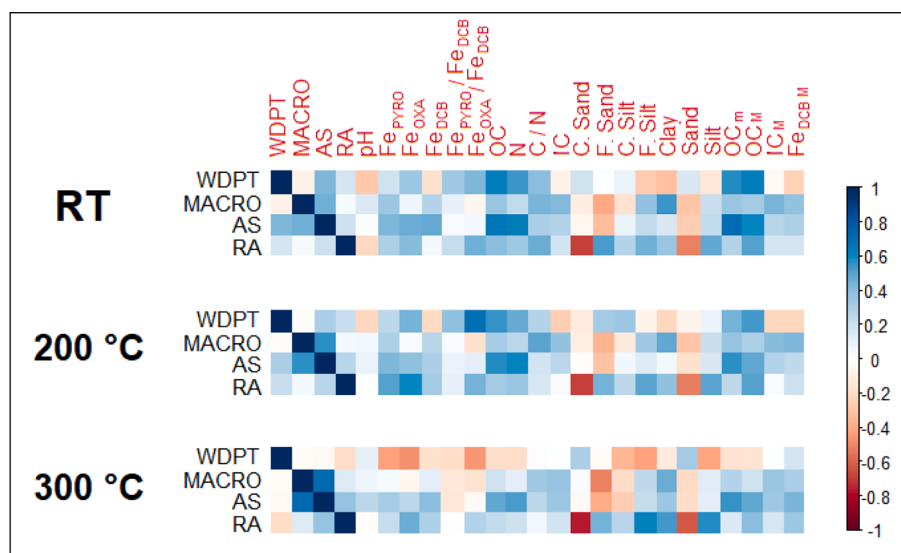
Fig. 5. Corrplot with red-to-blue colorbar (−1 to 1) at various temperatures (RT–200–300 °C).
