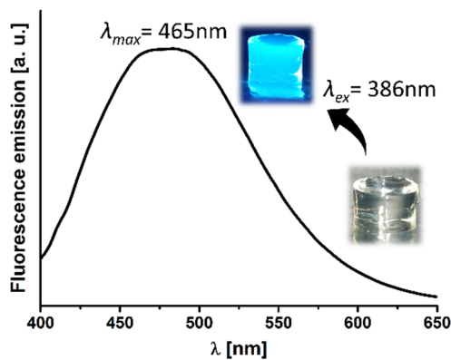
Fig. 2 Fluorescence emission spectra of ChDAT hydrogel upon excitation at 386 nm. Inset: Digital image of the hydrogel before and after UV light irradiation, showing its intrinsic fluorescence.
