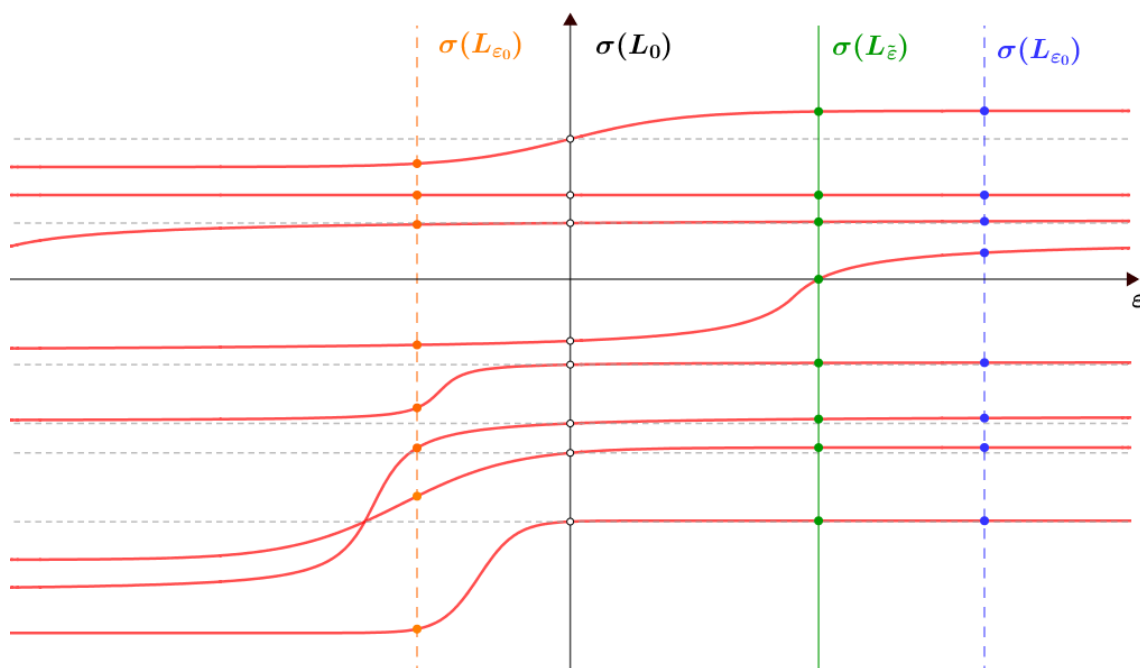
Figure 5 – Spectrum of L_\epsilon
