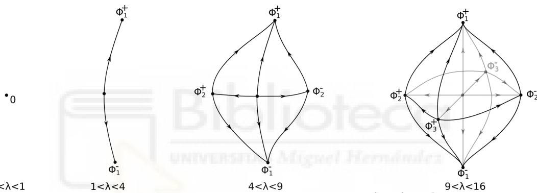
Figure 1 – Representations of the attractor for the Chafee-Infante problem, \lambda \in (0, 16) . Figures inspired by (HENRY, 1981, p. 5)
