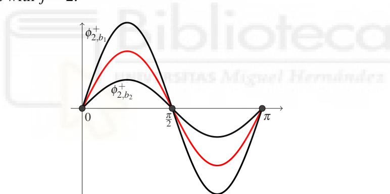
Figure 4 – A representation of the region X_2^+
