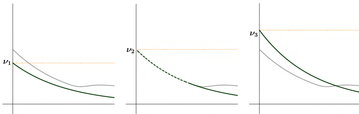
Figure 10 – Graphs of a_4 (in gray) and vc_1^\pm (in green) for different choices of v
