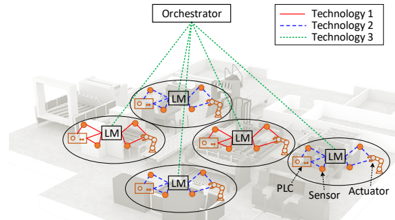
Fig. 1. Hierarchical and heterogeneous communications and data management architecture.
