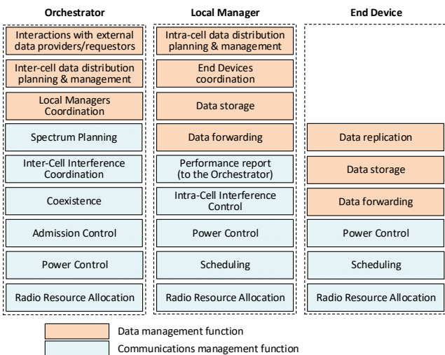
Fig. 2. Different communication and data management functions reside in different entities of the hierarchical architecture.
