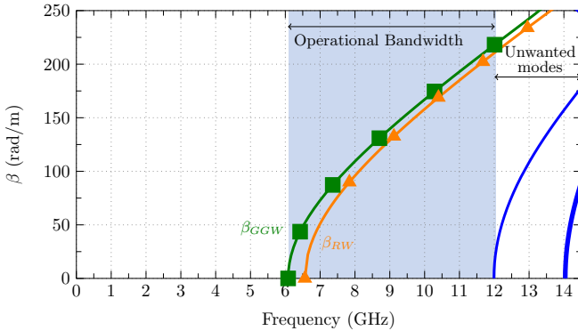
Fig. 2. Dispersion diagram of the GGW-90 (unwanted modes with solid lines and fundamental mode with square marks), and of the RW-90 RW (fundamental mode with triangle marks).
