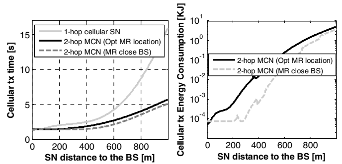
Fig. 5. Cellular tx : time the MR requires to transmit the data to the BS (left) and energy consumption (right).
