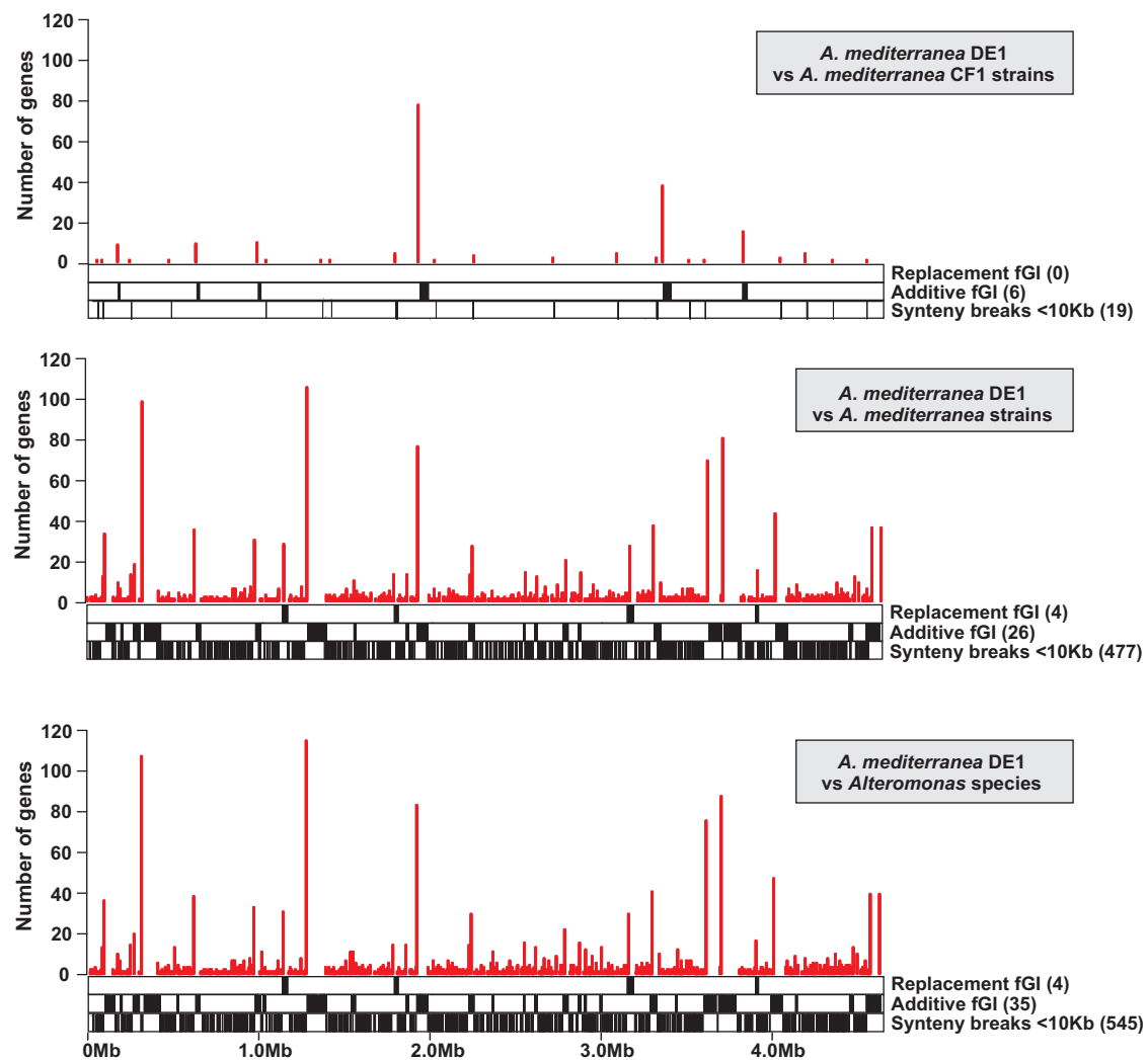
Fig. 4. —Synteny breaks for Alteromonas using A. mediterranea DE1 as a reference and comparing to genomes with increasing levels of divergence. Upper panel indicates synteny breaks within clonal frame 1, middle panel within A. mediterranea species and lower panel considering all the other strains in the genus. Vertical lines indicate gaps in the reference genome for which synteny is lost in any of the other genomes. Height of the line indicates the number of genes present in the reference strain that are not present in any of the others.
