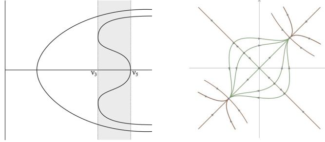
FIGURE 4. Expected structure of the attractor, when \nu \in (\nu_3, \nu_5) .
