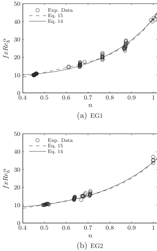
Fig. 10. Comparison between experimental results and experimental correlations.
