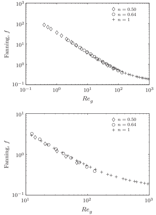
Fig. 12. EG2. Generalized Reynolds number Re_g (Eq. (18)) versus Fanning friction factor.
